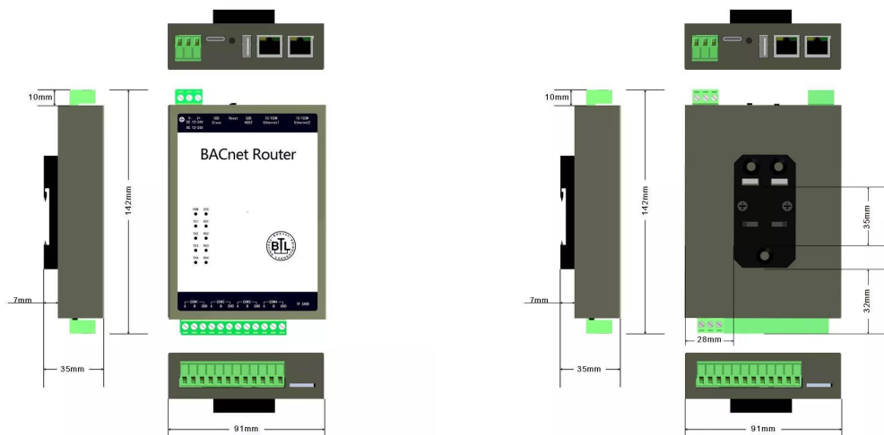
Router2004-A9 (DIN-Rail)
